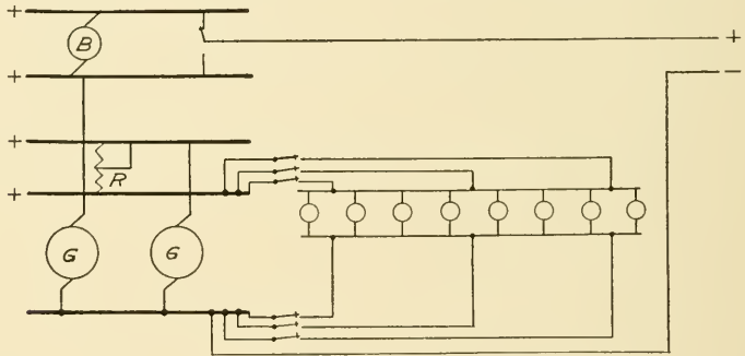
Fig. 11. Diagram of Connections for Voltage Regulation
